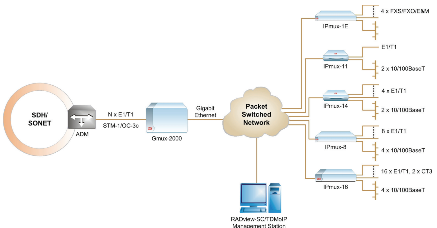
Figure 1. RADview-SC/TDMoIP Managing Pseudowire Devices in a Typical TDMoIP Application
