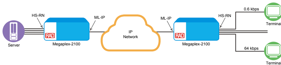
Figure 1. Point-to-Point Low Speed Data Connection
