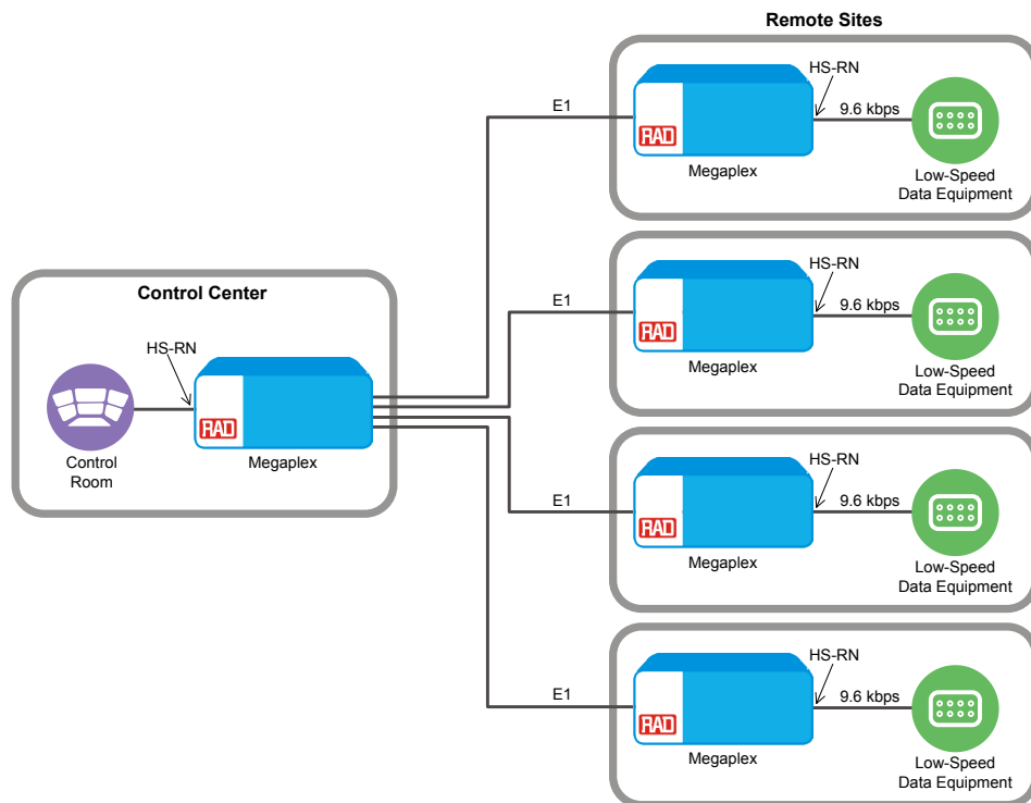
Figure 2. Point-to-Multipoint Connectivity at Low-Speed Data Transfer
